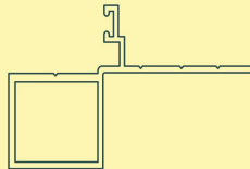
DJ3260 Jamb Adaptor
