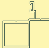
DJ3250 Jamb Adaptor
